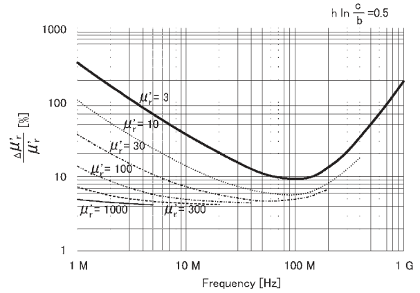
Figure 22. Permeability accuracy \left(\frac{\Delta\mu_r'}{\mu_r'}\right) vs. frequency (at F = 0.5 , typical)
