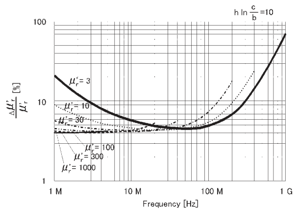
Figure 24. Permeability accuracy \left(\frac{\Delta\mu_r'}{\mu_r'}\right) vs. frequency (at F = 10 , typical)
